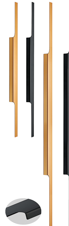
5759 孔距: 300/350/400/450/500/600/800 1000/1500/2000/2200/2500mm/ 2800mm(1.5米以上分左右)
